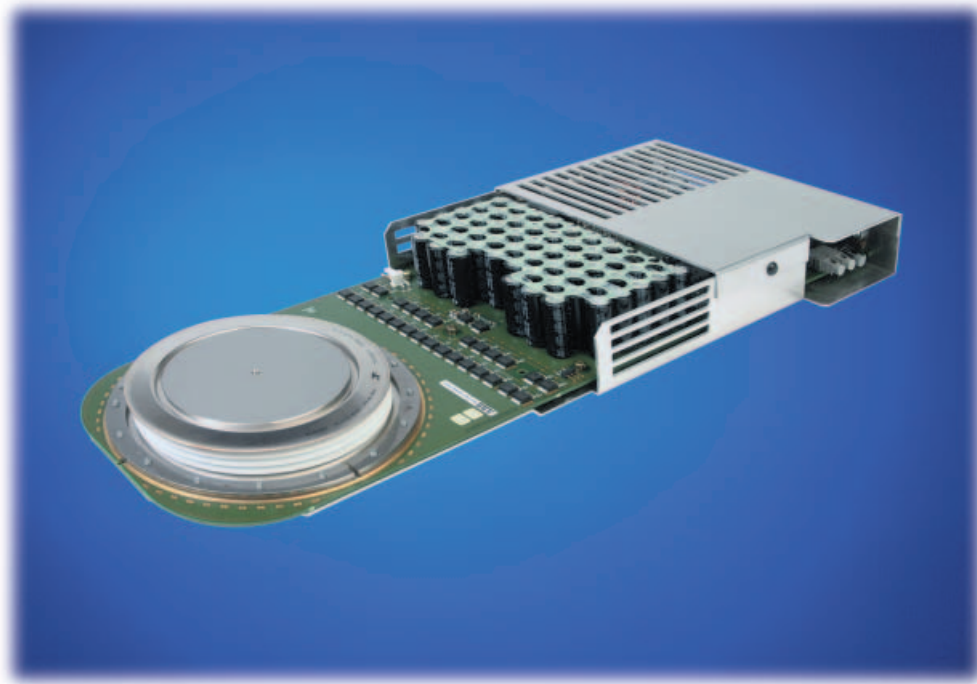
IGCT type 5SHY 55L4500 – 91 mm, 4.5 kV
