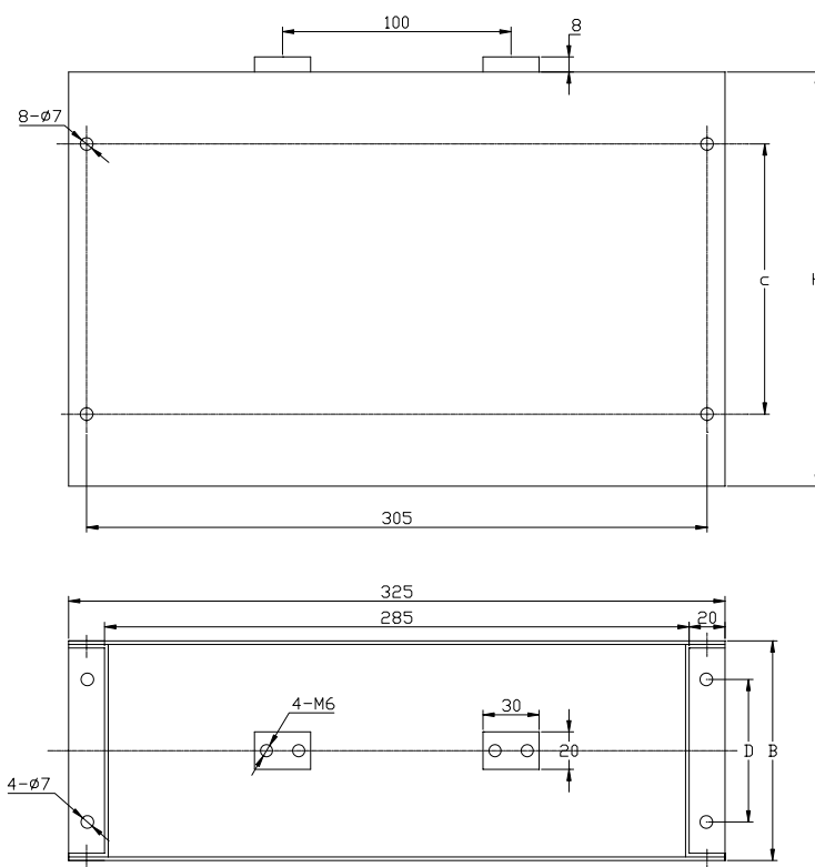
Case code : dimensions in mm
